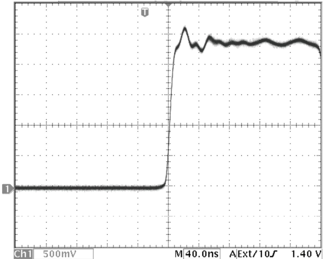
Figure 6.1 Rise Time 10x attenuation, 10%-90%
