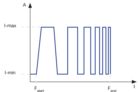
Sweep mode load profile
