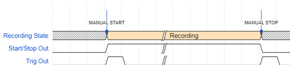
FIGURE 3.35 : Chronogramme Start / Stop
