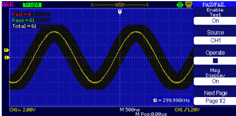
Figure 3.64 – Pass/Fail Screen 1
