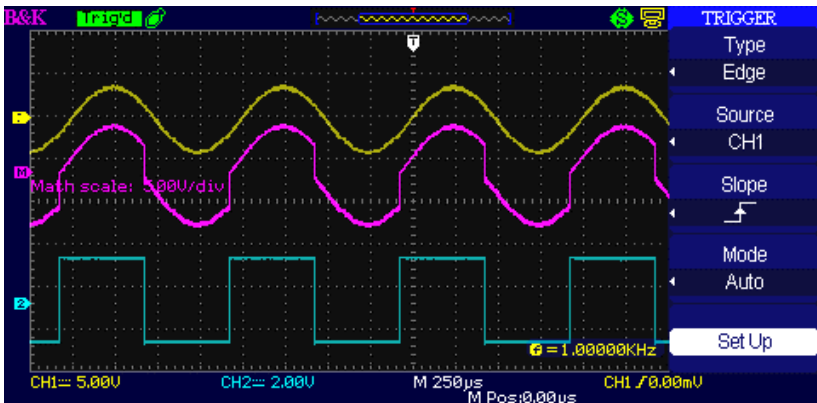
Figure 3.15 – Math Waveform
