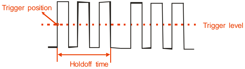
Figure 3.30 – Trigger Holdoff Illustration
