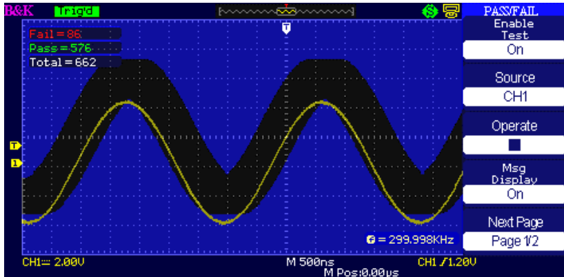
Figure 3.65 – Pass/Fail Screen 2
