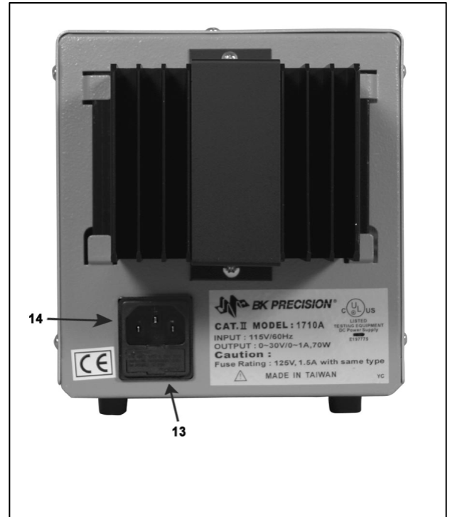
Figure 2. Rear Panel
