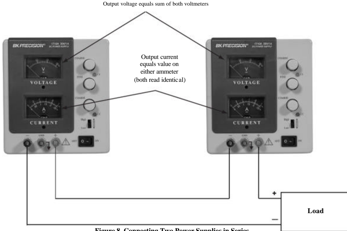
Figure 8. Connecting Two Power Supplies in Series.
