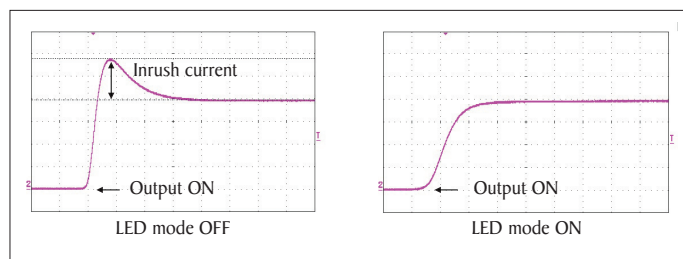
Current flow during power up with LED mode enabled
